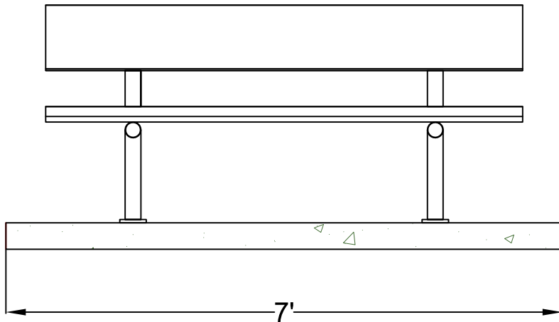
1 Park Bench & Concrete Pad - Front View
