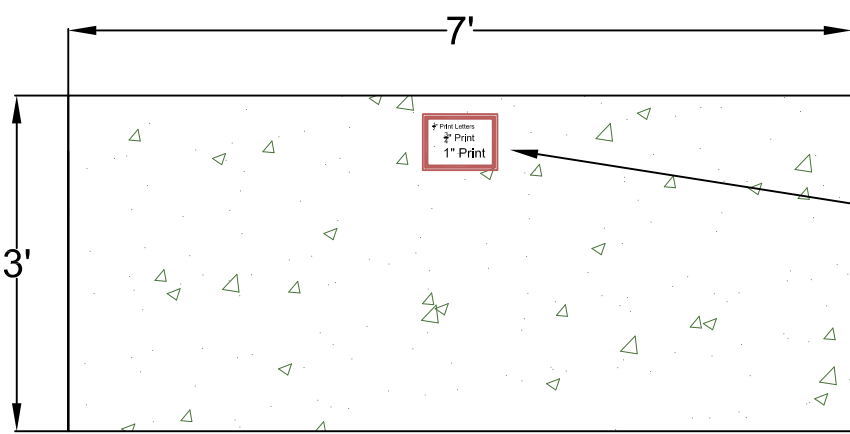
2 Concrete Pad - Top View
